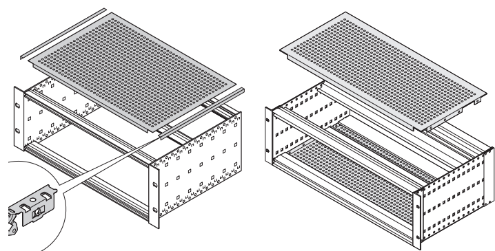
Universal EMC cover plate
