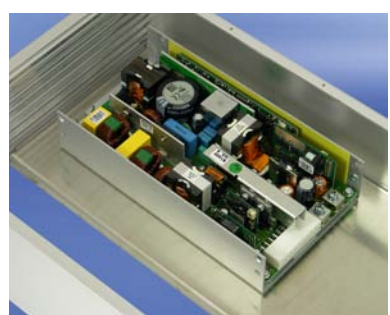
Mounting plate for installation of heavy components
