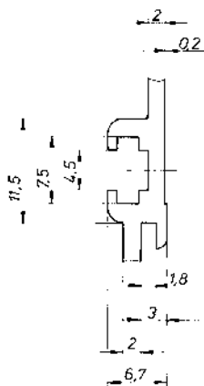
Detail "Y"
