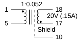
Schematic 7
