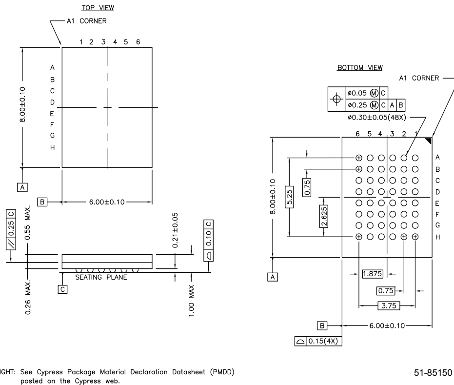
Figure 17. 48-ball VFBGA (6 × 8 × 1.0 mm) BV48/BZ48 Package Outline, 51-85150
