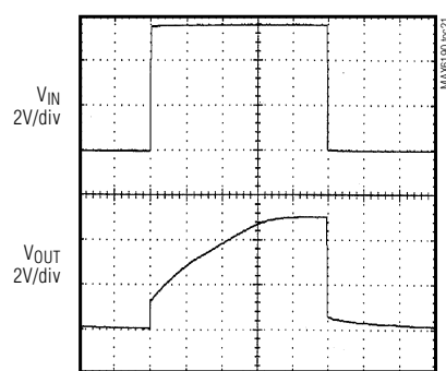
MAX6195 TURN-ON TRANSIENT
