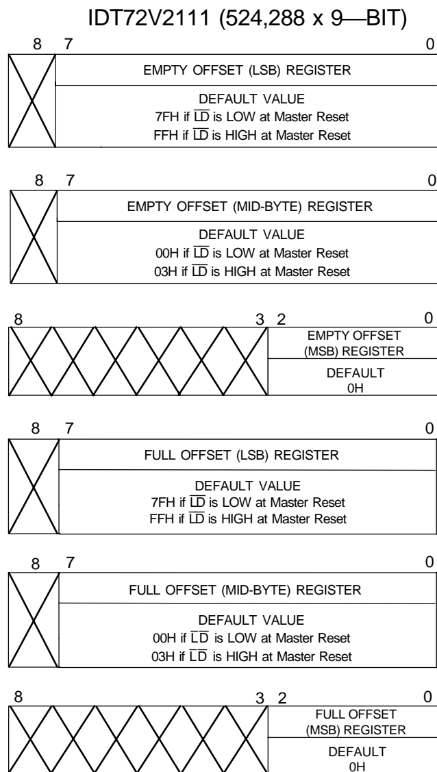
Figure 3. Offset Register Location and Default Values
