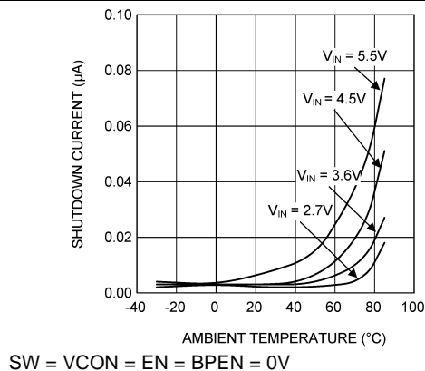
Figure 1. Shutdown Current vs Temperature
