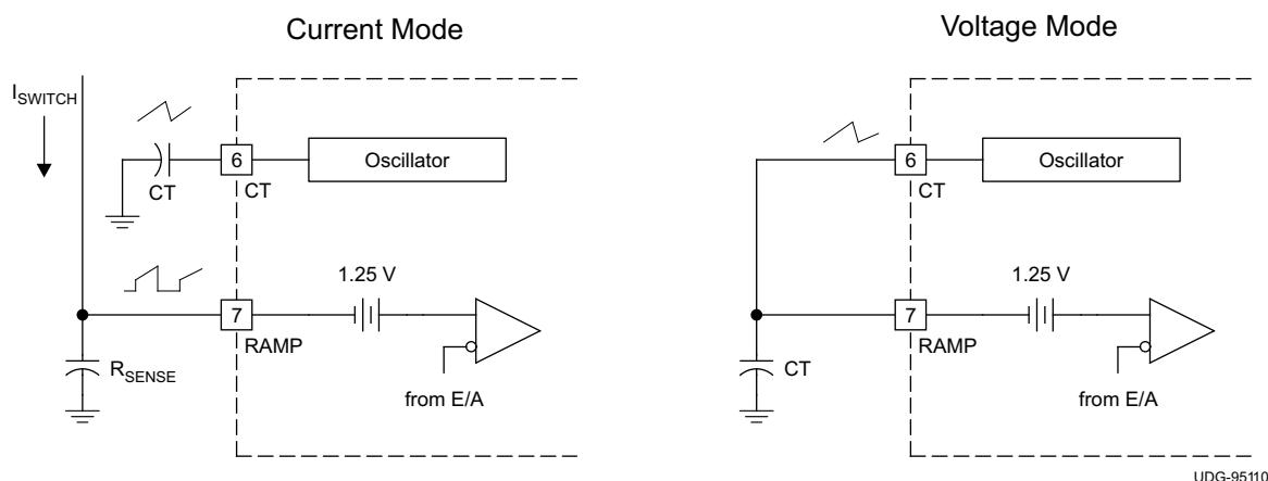
Figure 7. Control Methods
