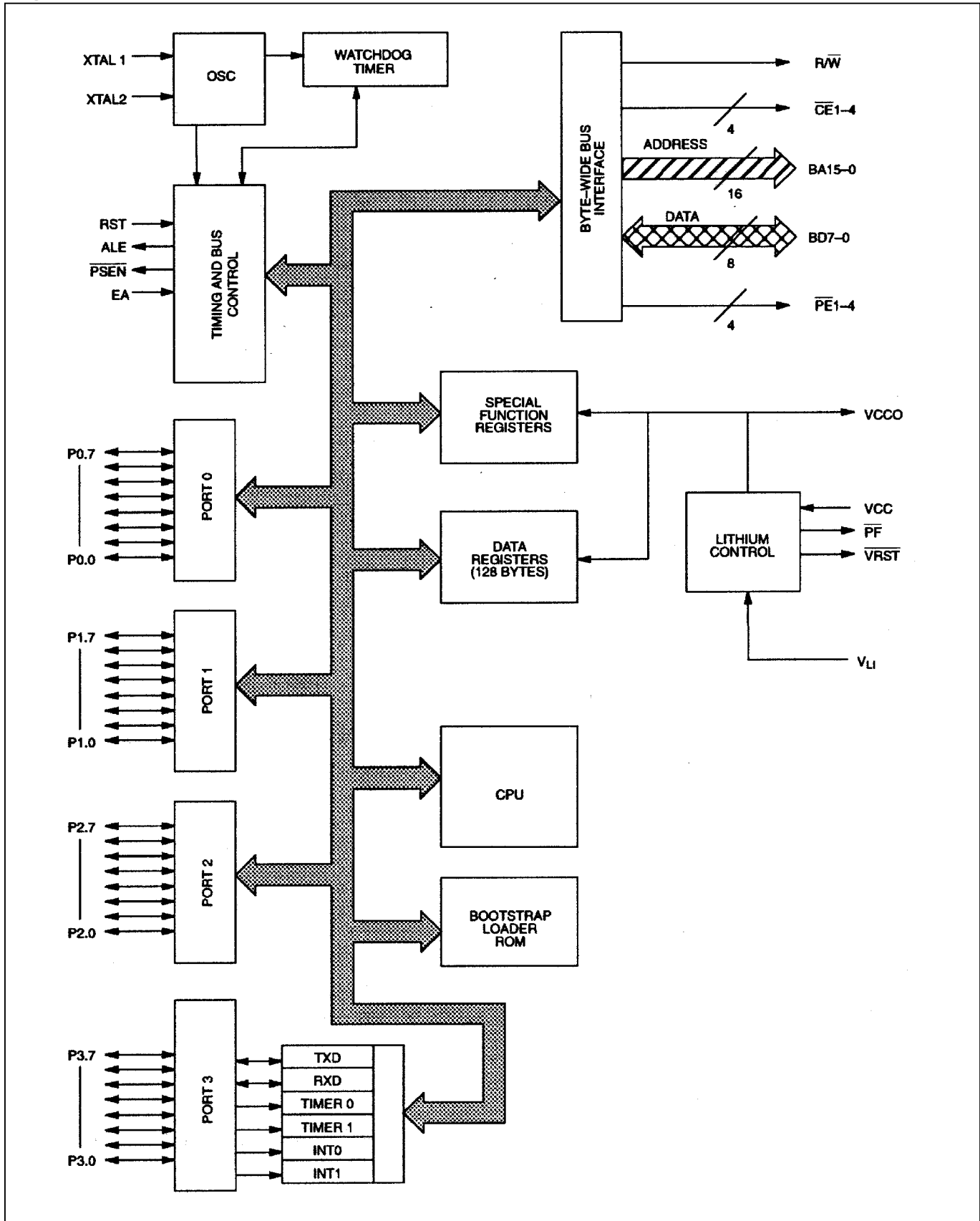
Figure 1. BLOCK DIAGRAM
