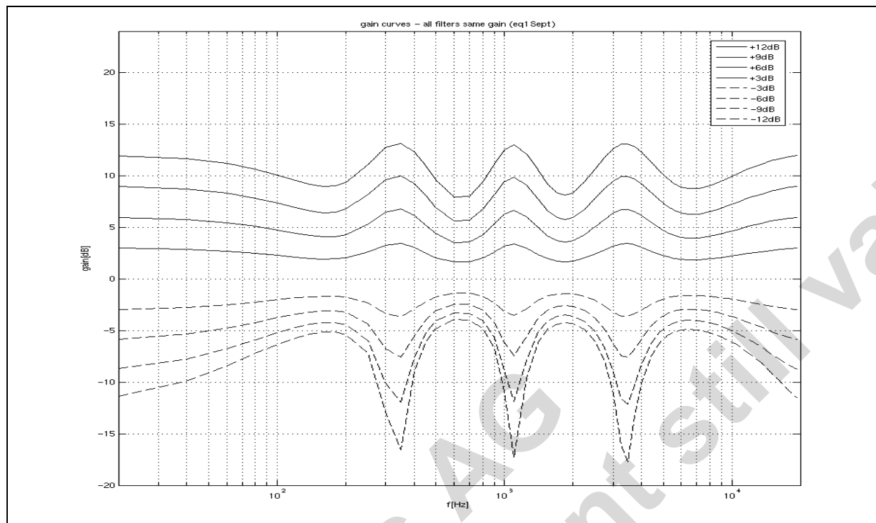
Figure 46. EQ Filter frequency response sum curve
