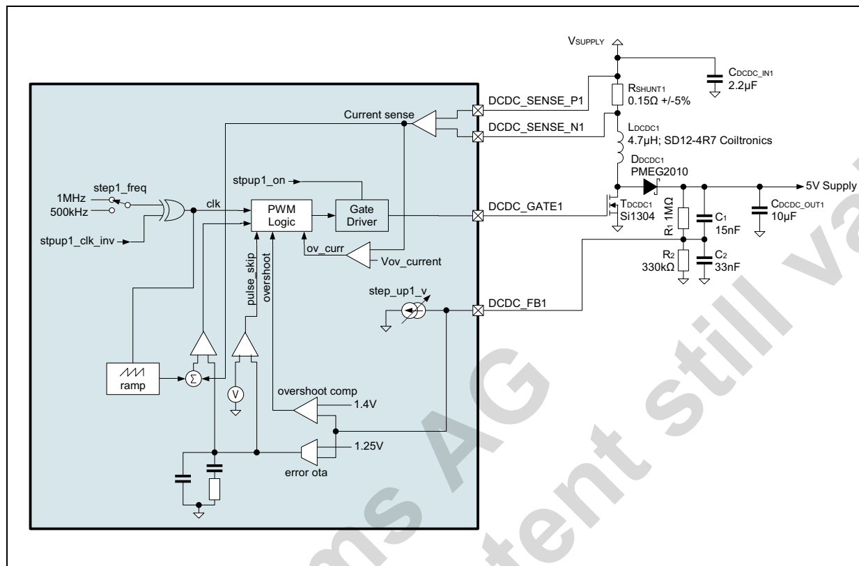
Figure 6. DC/DC step up 1 converter with regulated output voltage of 5V. Feedback is at pin DCDC_FB1
