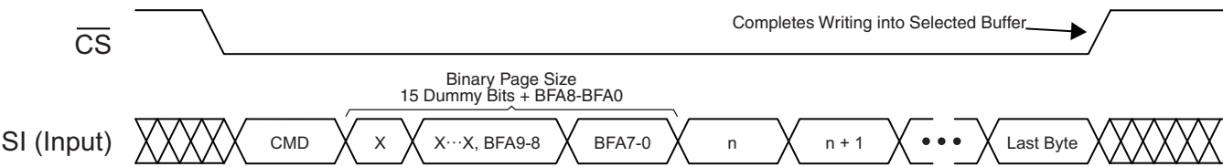
Figure 23-2. Buffer Write
