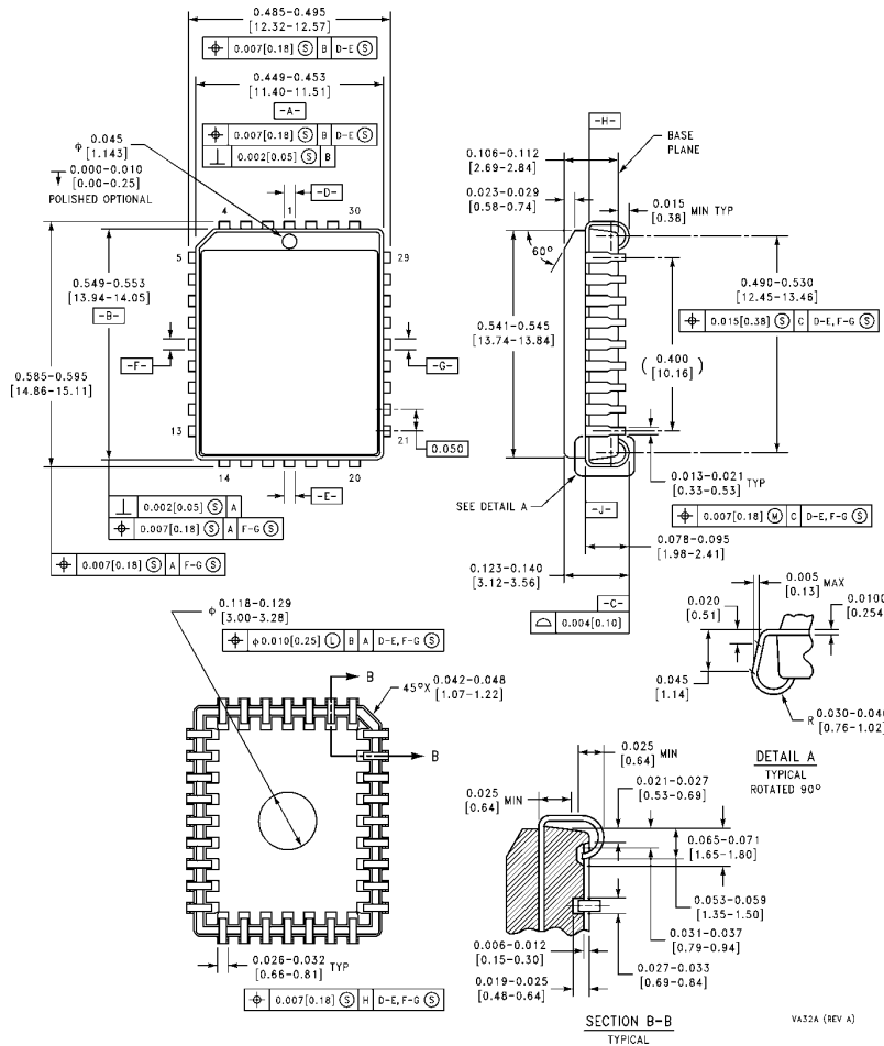
32-Lead Plastic Leaded Chip Carrier (PLCC)
