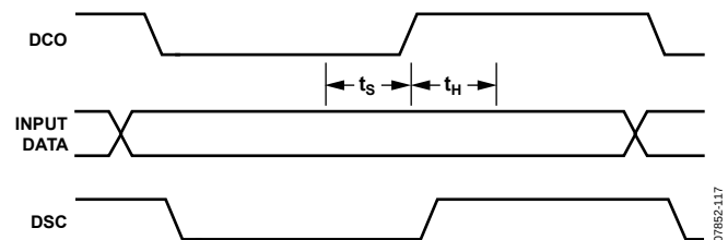
Figure 100. CMOS Input Timing
