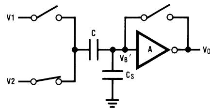
FIGURE 6. Sampled-Data Comparator
