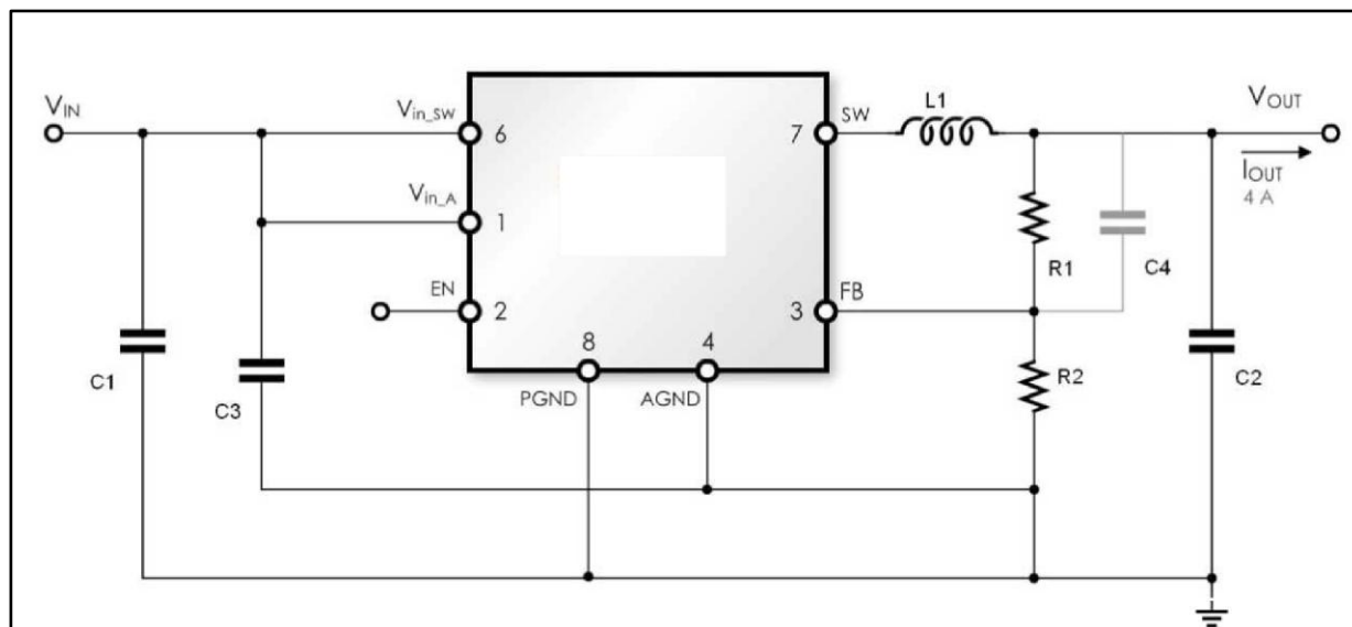
Figure 1: Application schematic
