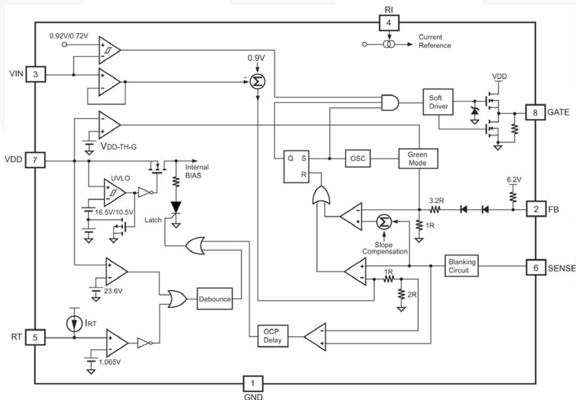
Figure 2. Block Diagram
