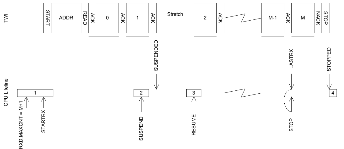
Figure 109: The TWI master reading data from a slave
