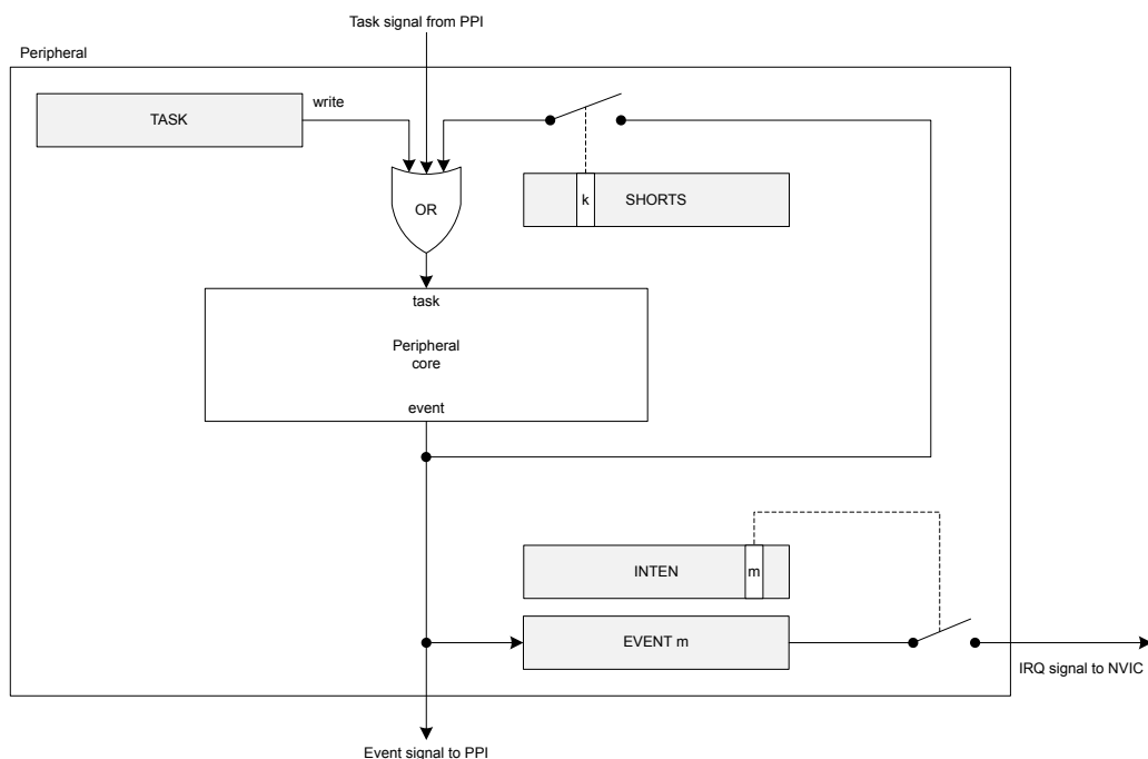
Figure 21: Tasks, events, shortcuts, and interrupts
