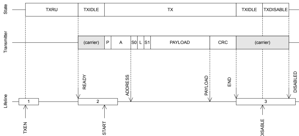
Figure 63: Transmit sequence
