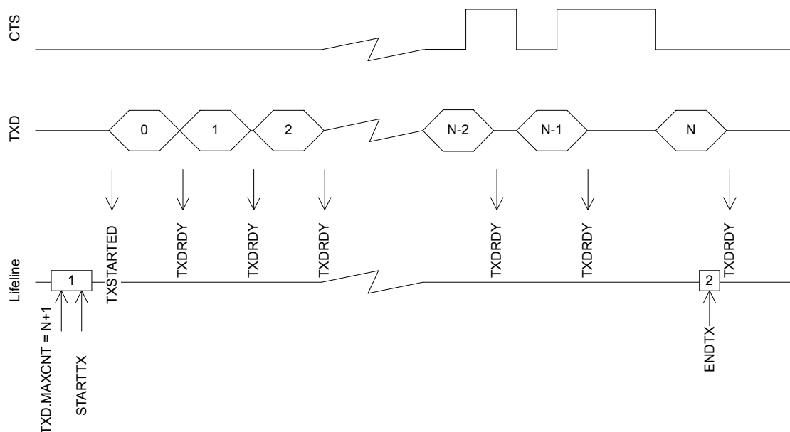
Figure 122: UARTe transmission
