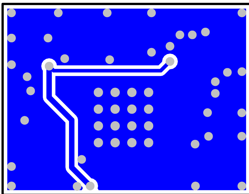
Figure 135: Bottom layer
