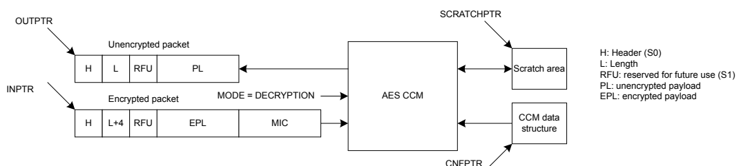
Figure 28: Decryption
