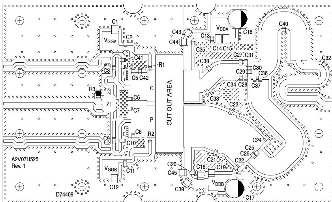
Figure 24. A2V07H525-04NR6 Test Circuit Component Layout — 758–803 MHz
