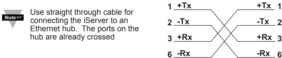
Figure 2.7 10Base-T Crossover Cable Wiring
