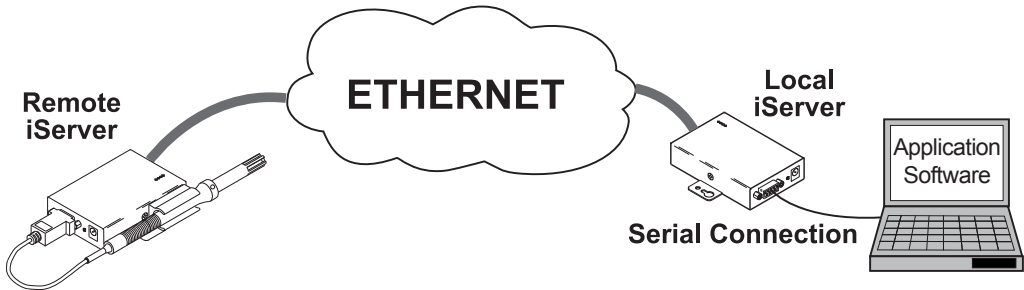
Figure 4.14 PC-to-Device Communication
