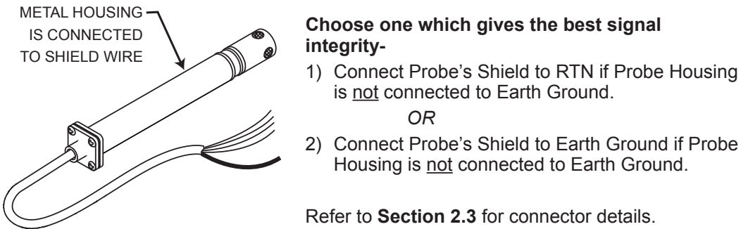
Figure 2.8 Industrial Probe Wiring Hookup
