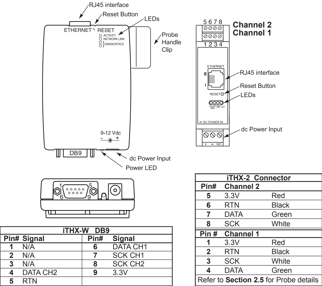
Figure 2.5 Parts of the iServer Unit
