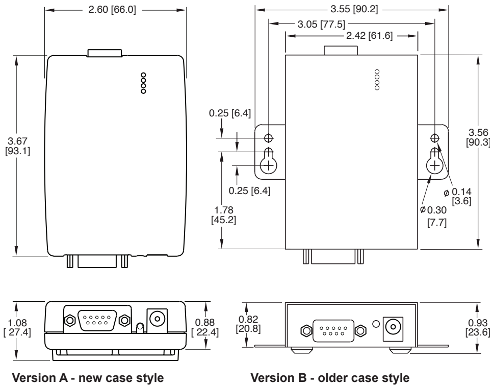
Figure 5.1 Wall Mount iServer Dimensions
