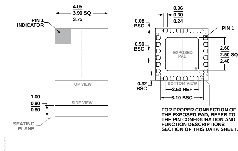
Figure 34. 24-Terminal Ceramic Leadless Chip Carrier [LCC] (E-24-1)
