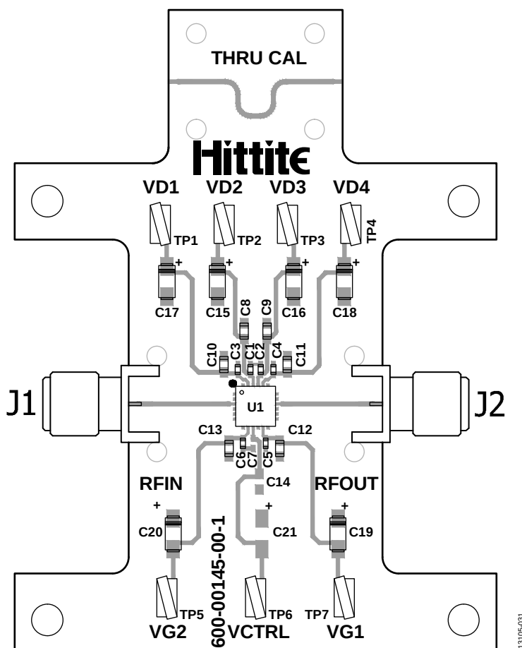
Figure 32. 600-00145-00-1 Evaluation PCB
