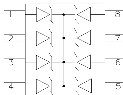
SO-8 (Top View)
