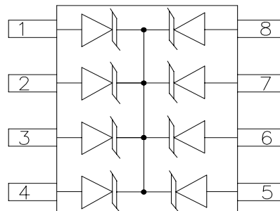
Circuit Diagram
