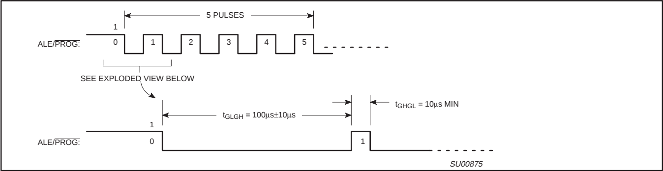
Figure 42. PROG Waveform
