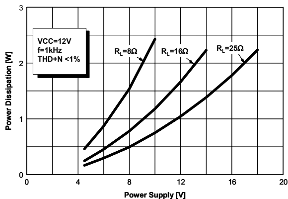
Fig. 8 Power Dissipation vs. Supply Voltage
