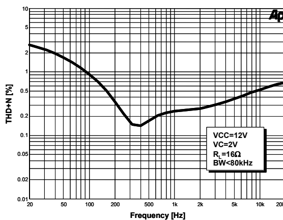
Fig. 4 THD+N vs. Frequency
