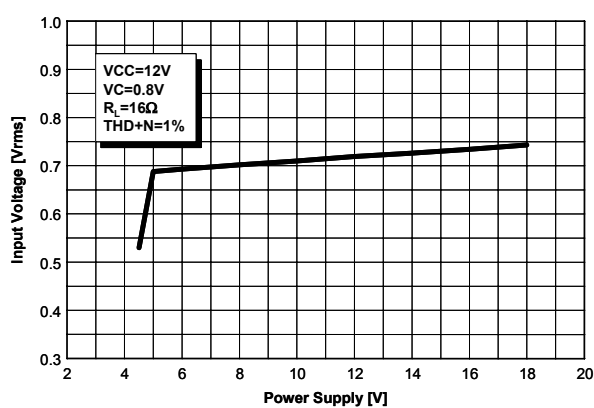
Fig. 6 Input Signal Handling
