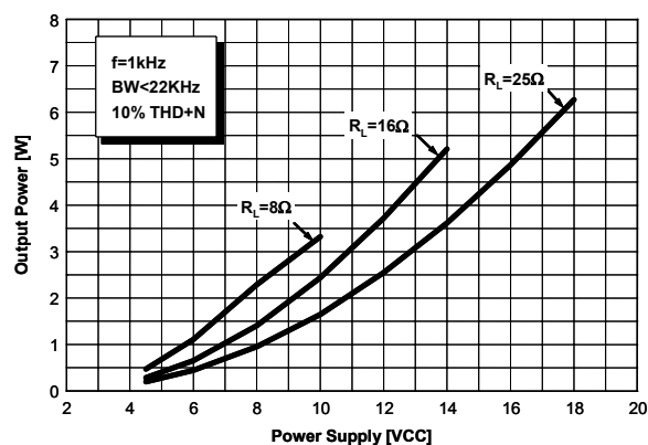
Fig. 12 Output Power vs. Supply Voltage
