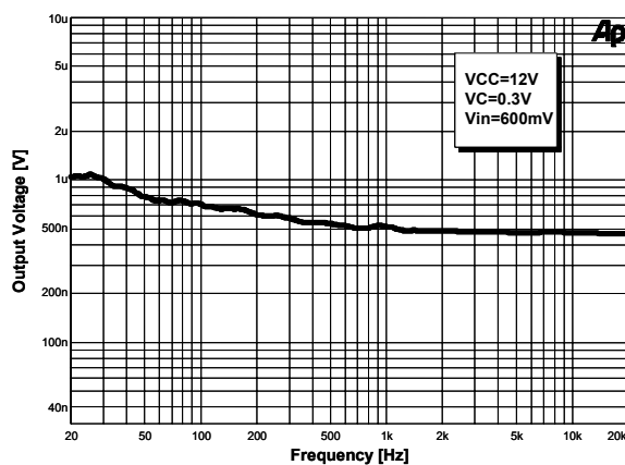
Fig. 14 Output Voltage in Mute State
