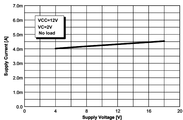
Fig. 1 Supply Current
