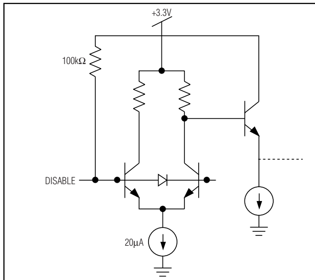
Figure 4. TTL Input Stage
