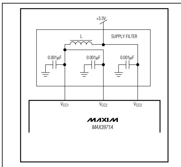
Figure 5. Power-Supply Filter
