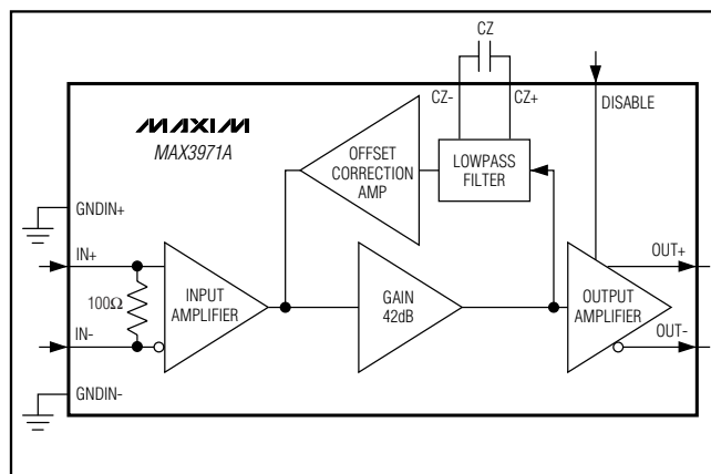
Figure 1. Functional Diagram
