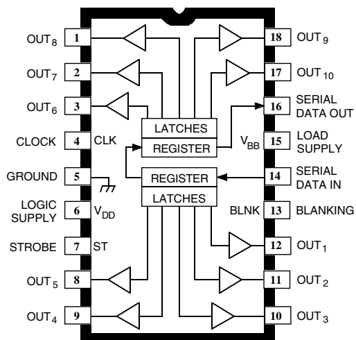
UCN5810AF
