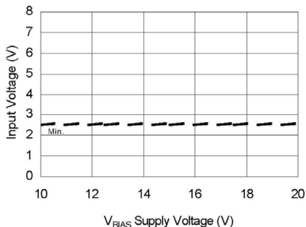
Figure 12B. Logic "1" Input Voltage vs. Voltage
