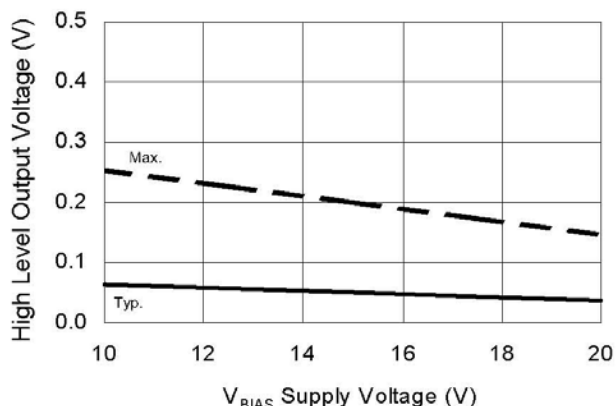
Figure 14B. High Level Output vs. Supply Voltage
