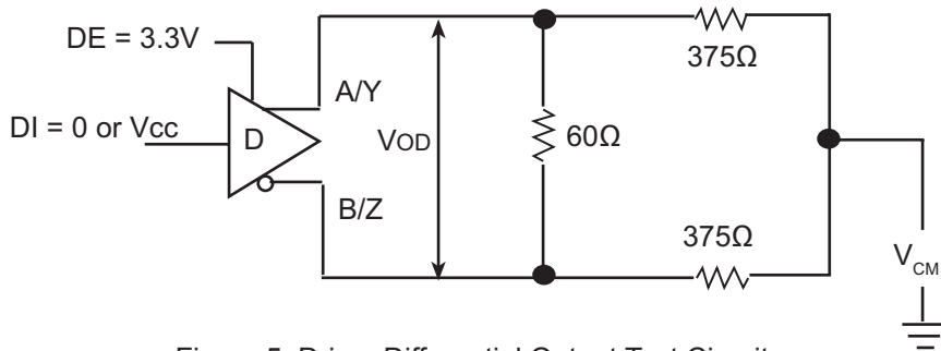
Figure 5. Driver Differential Output Test Circuit
