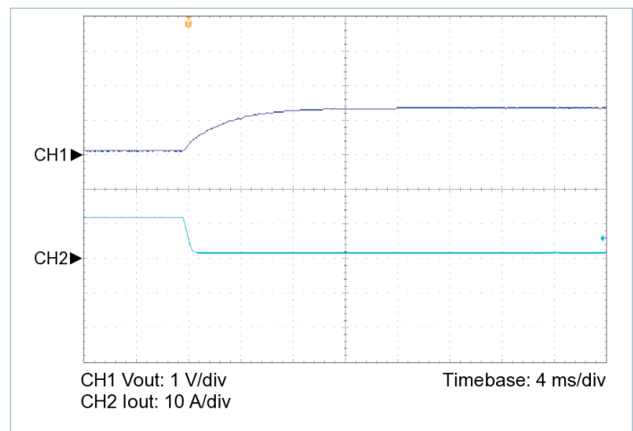
Figure 7 — 100% to 10% load transient response, V_{IN} = 24\text{ V} , nominal trim, C_{OUT\_EXT} = 1000\text{ }\mu\text{F}
