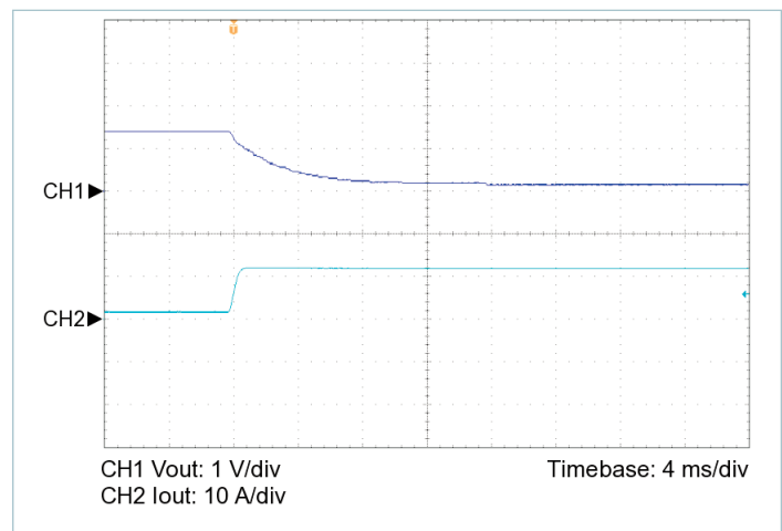
Figure 8 — 10% to 100% load transient response, V_{IN} = 24\text{ V} , nominal trim, C_{OUT\_EXT} = 1000\text{ }\mu\text{F}
