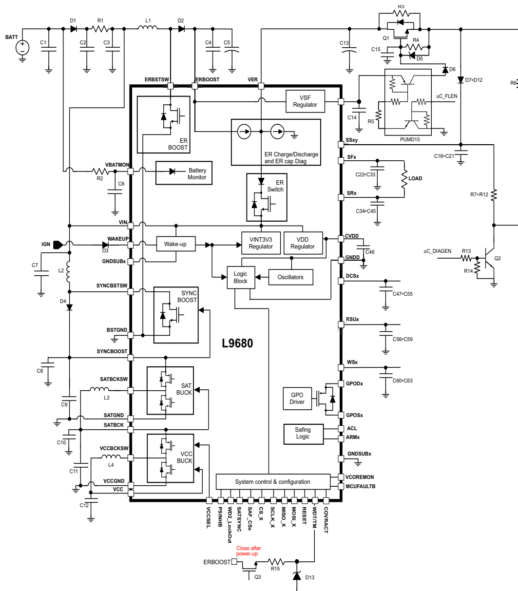
Figure 71. Application circuit
