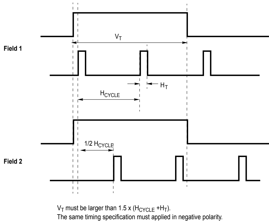
Figure 16 H_{\text{SYNC}} and V_{\text{SYNC}} Specification
