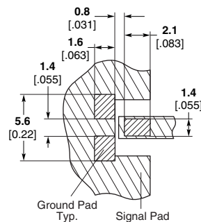
Recommended Mounting Pattern
