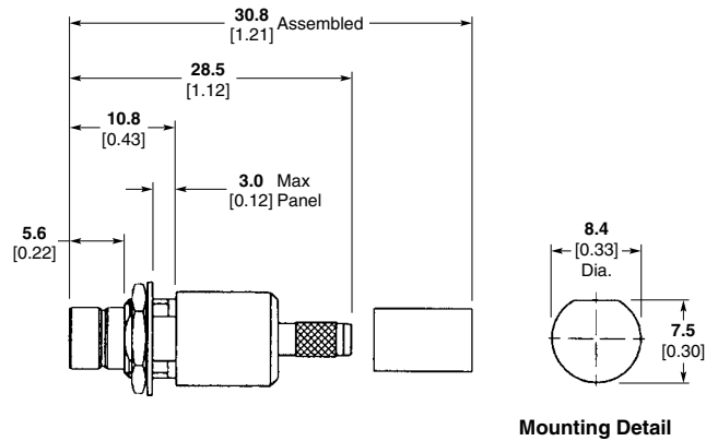
Mounting Detail
