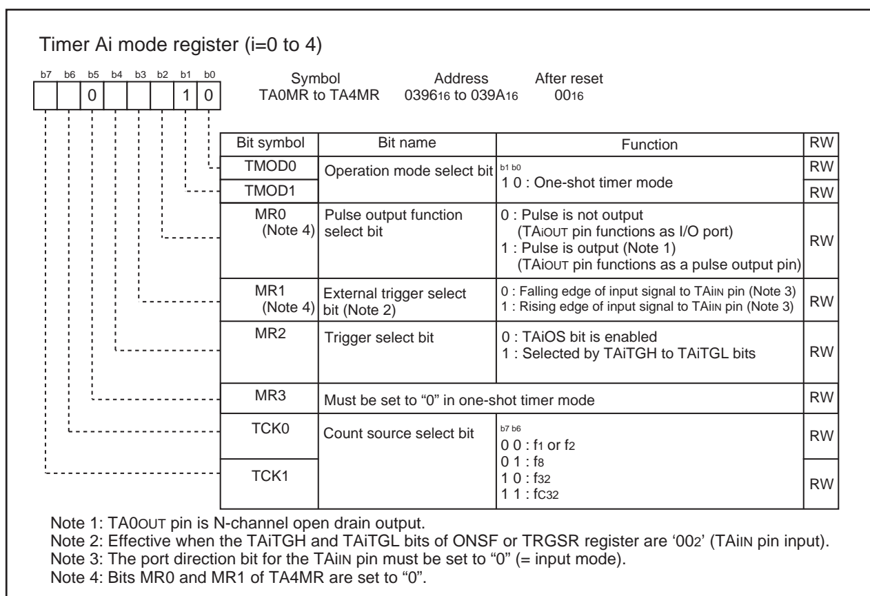
Figure 10.11. TAIiMR Register in One-shot Timer Mode
