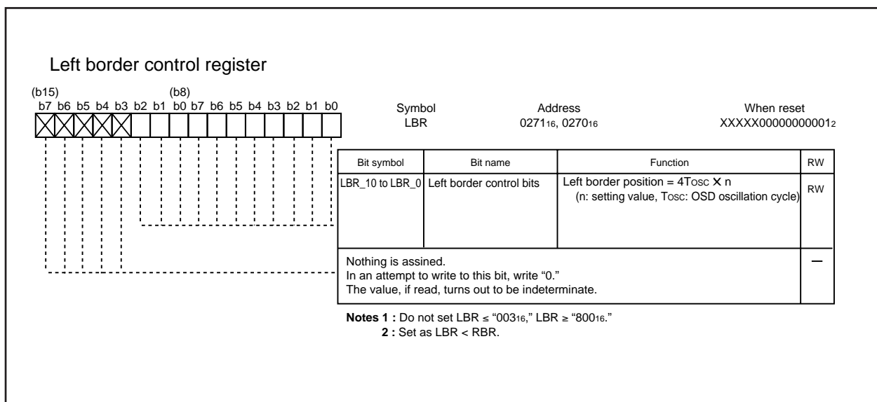
Figure 16.48 Left border control register
