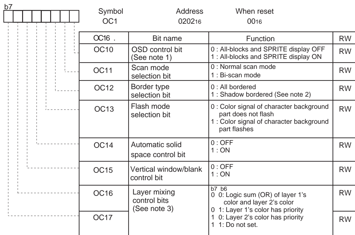
OSD control register 1
