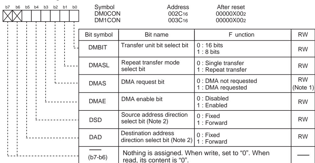
DMAi control register(i=0,1)
