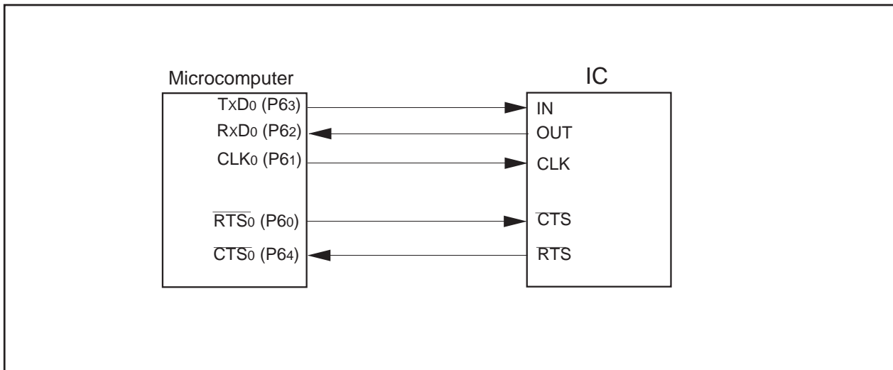
Figure 11.14. CTS/RTS Separate Function
