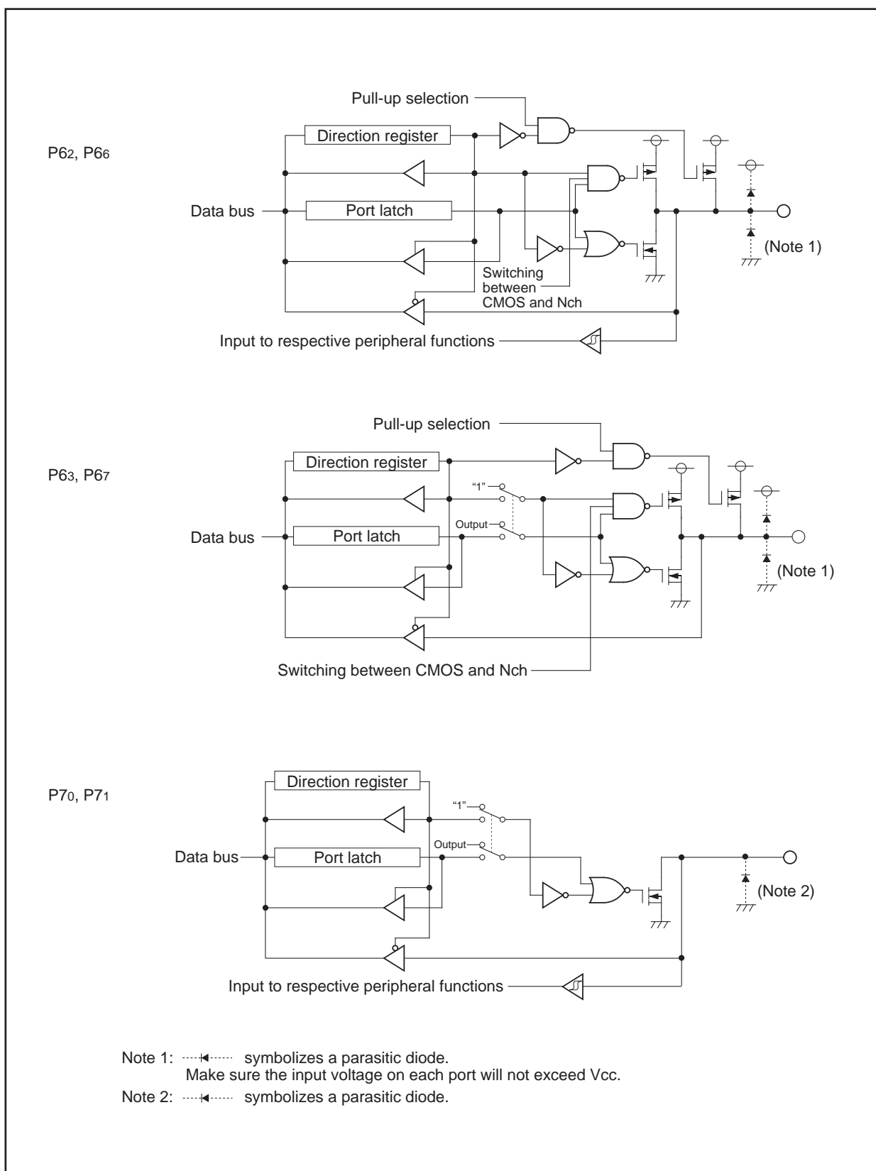
Figure 17.3. I/O Ports (3)
