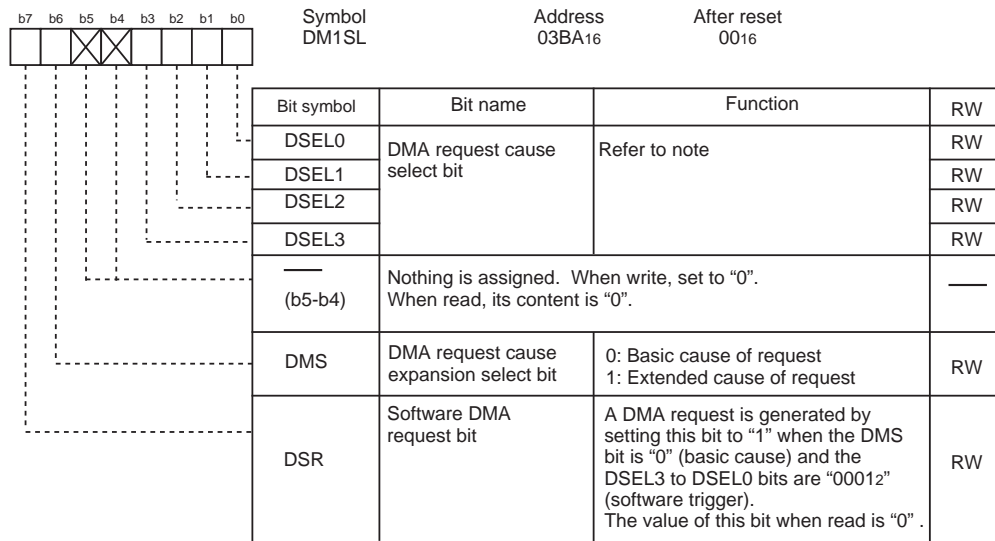
DMA1 request cause select register
