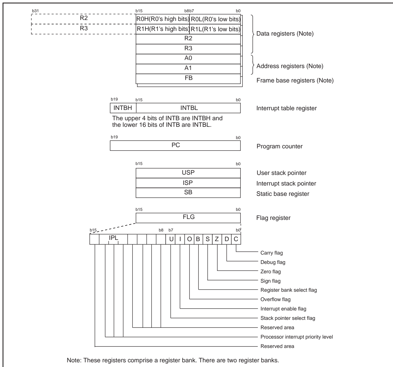
Figure 2.1. CPU registers
