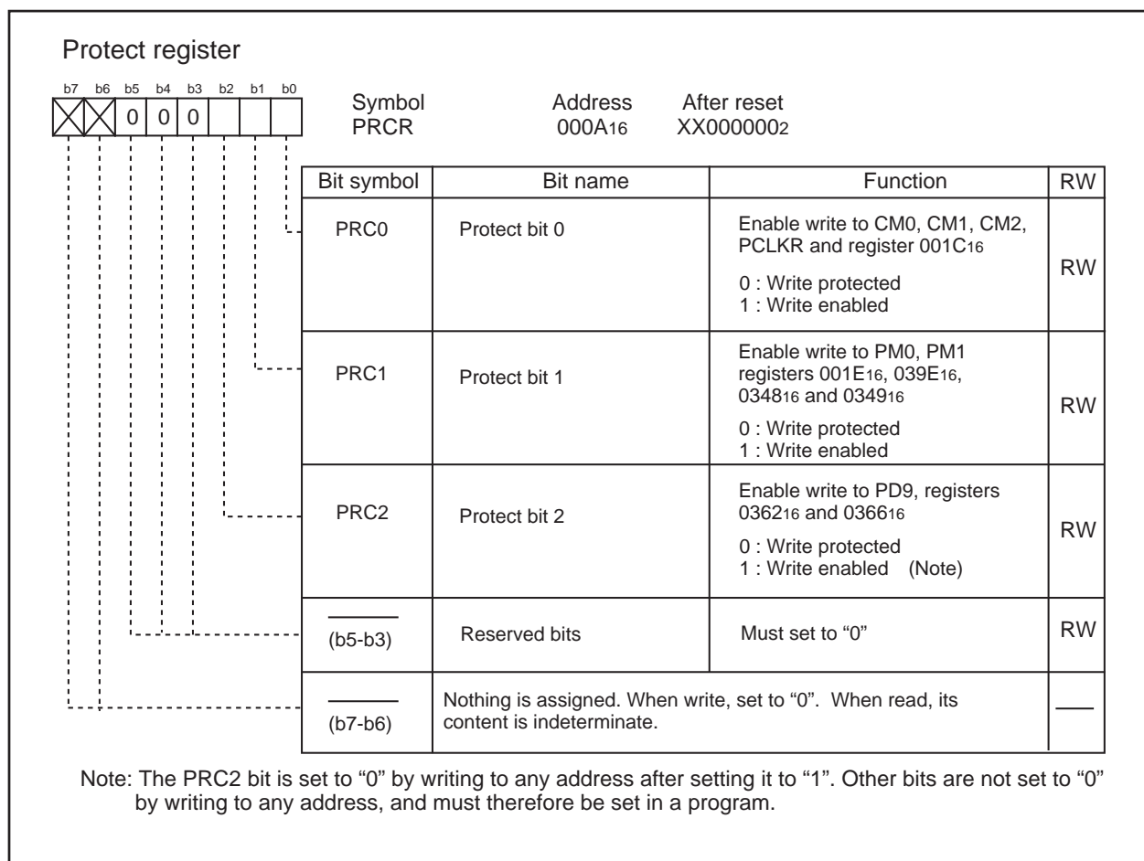
Figure 6.1. PRCR Register
