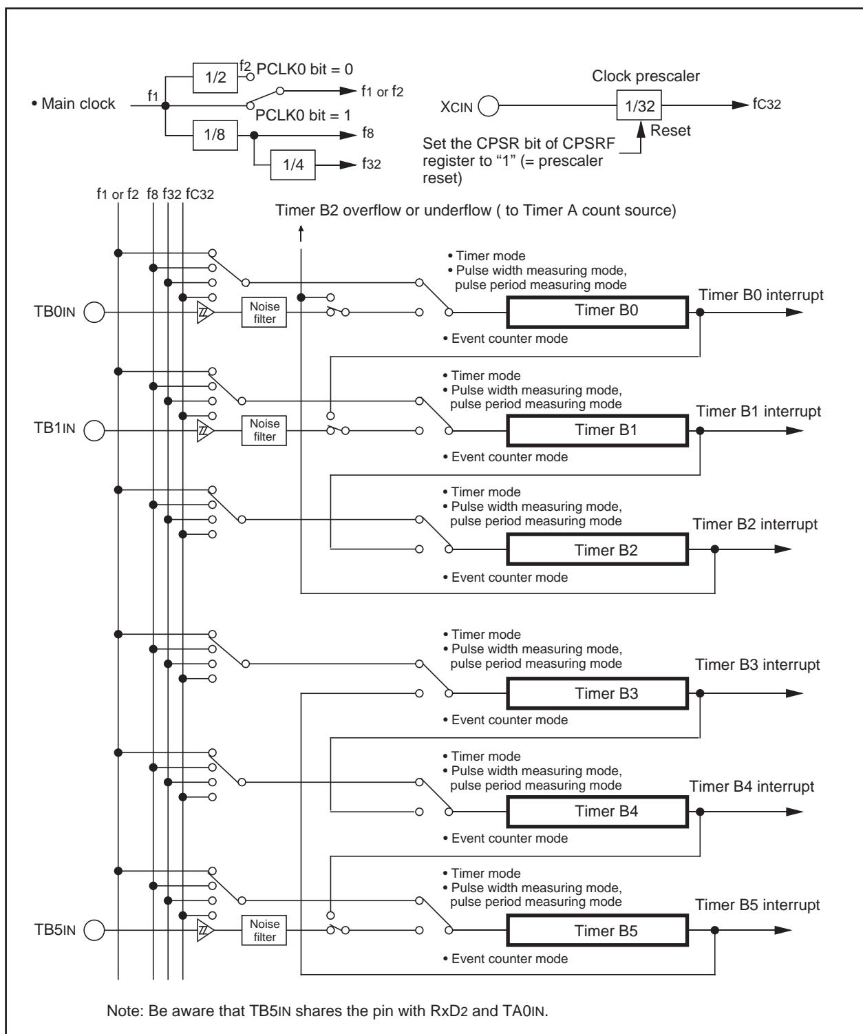
Figure 10.2. Timer B Configuration
