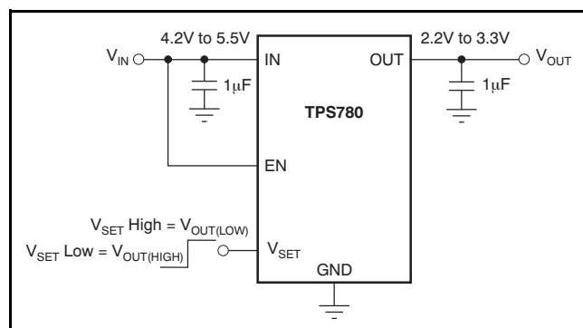
Figure 58. Circuit Showing EN Tied High when Shutdown Capability is Not Required
