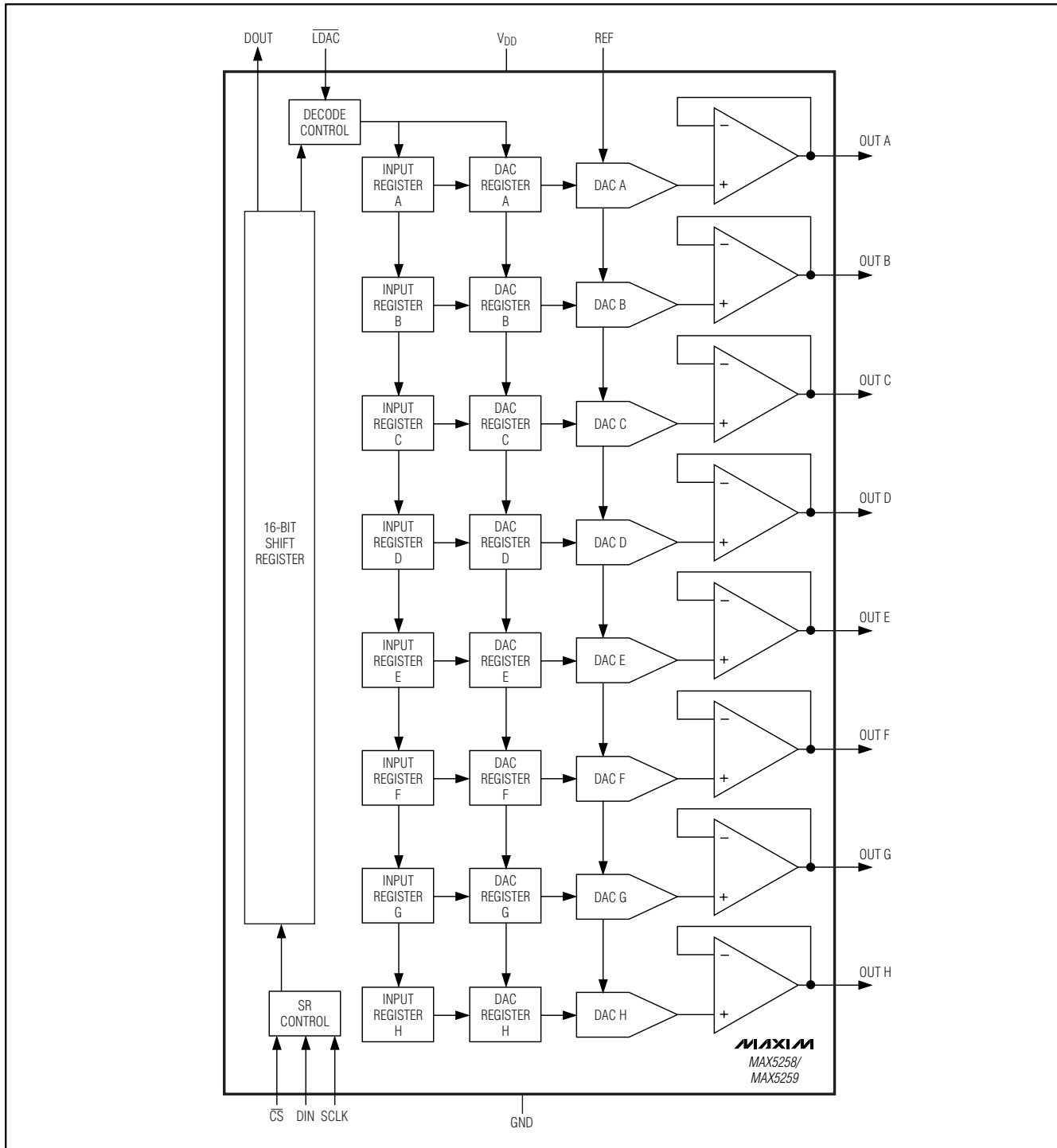
Functional Diagram
