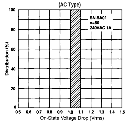
Distribution of On-State Voltage Drop
