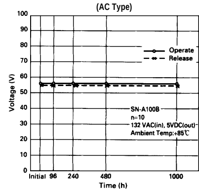
High temperature Continuous Operating Test
