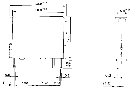
SN-A ( ) type (output module)
