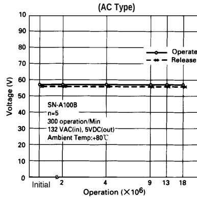
High temperature Switching Test
