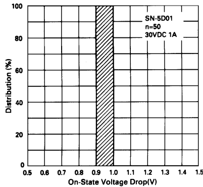
Distribution of On-State Voltage Drop
