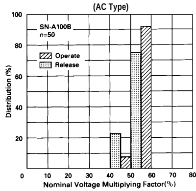
Distribution of Operate & Release Voltage
