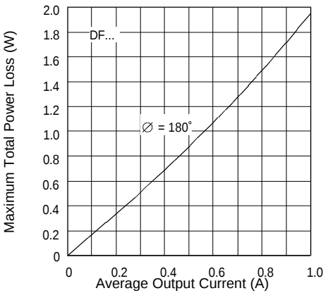
Fig. 2 - Power Loss Characteristics
