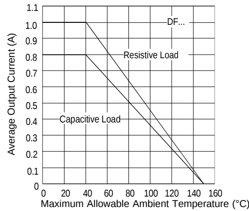
Fig. 3 - Current Ratings
