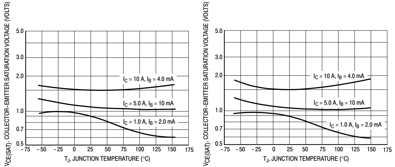
Figure 4. Collector-Emmitter Saturation Voltage
