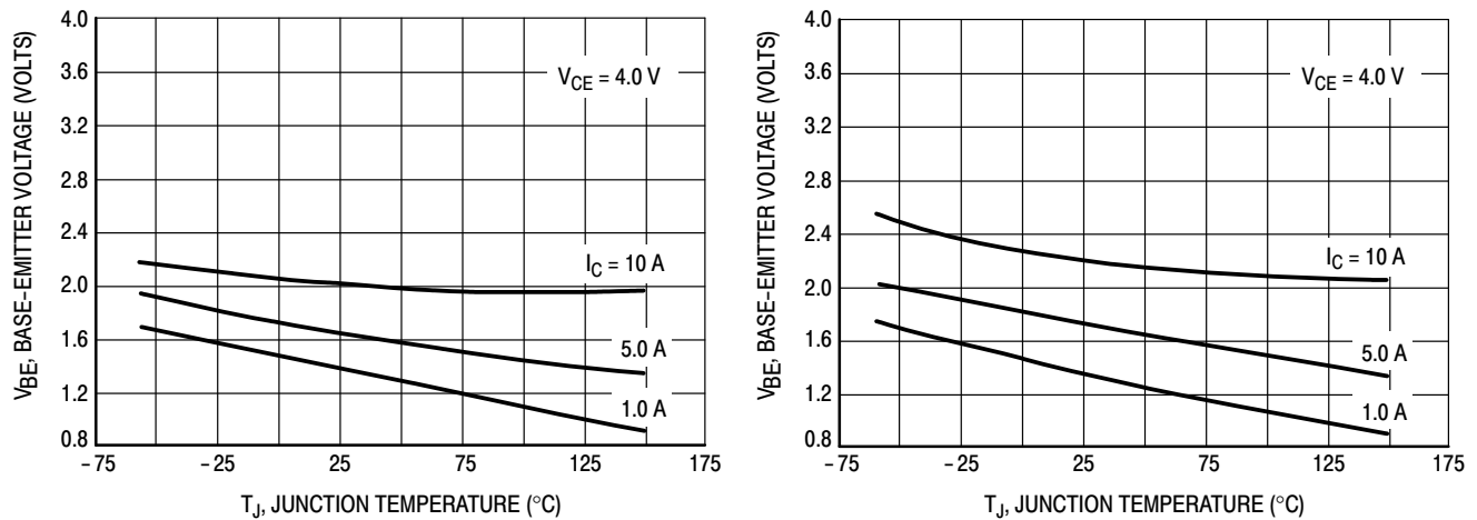
Figure 5. Base-Emmitter Voltage
