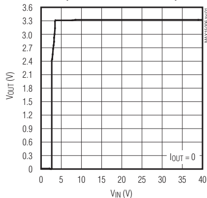
OUTPUT VOLTAGE vs. INPUT VOLTAGE (MAX15006A/MAX15007A)
