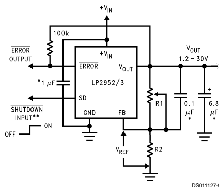
FIGURE 4. Adjustable Regulator
