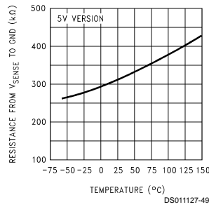
Divider Resistance
