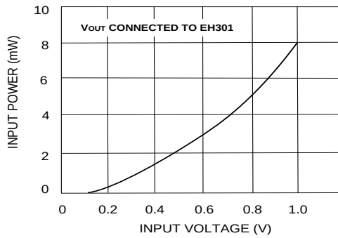
INPUT POWER AS A FUNCTION OF INPUT VOLTAGE
