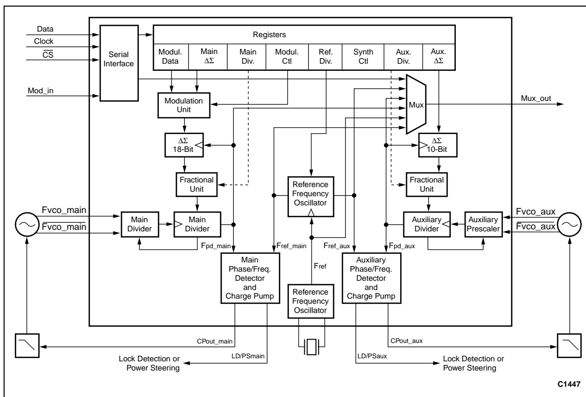
Figure 1. CX72302 Functional Block Diagram
