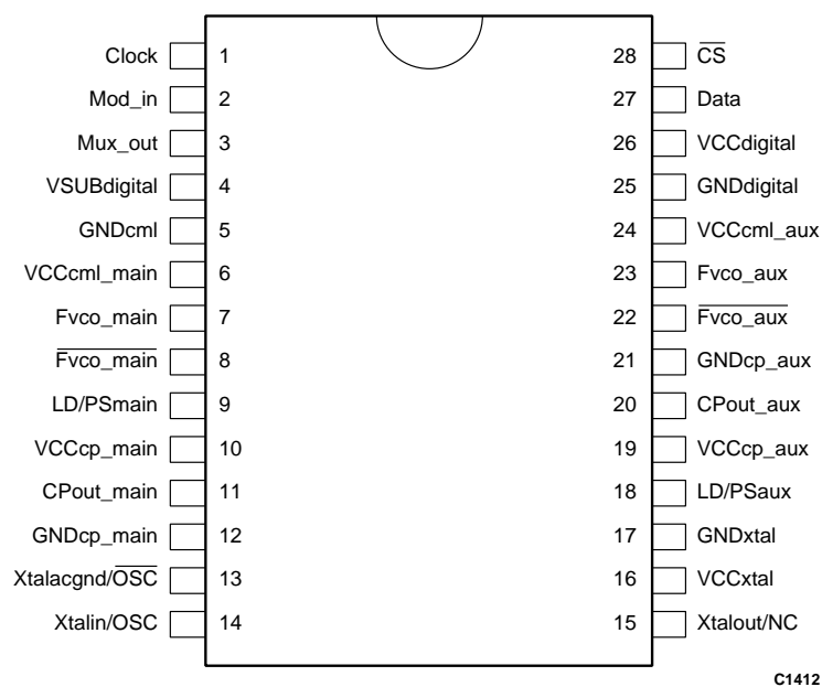
Figure 2. CX72302 Pinout, 28-Pin EP-TSSOP
