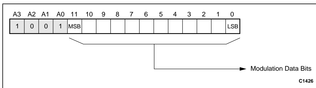
Figure 15. Modulation Data Register (Write Only)
