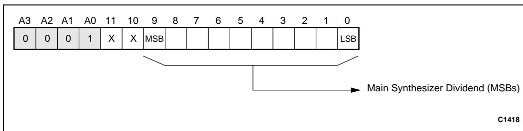
Figure 7. Main Dividend MSB Register (Write Only)
