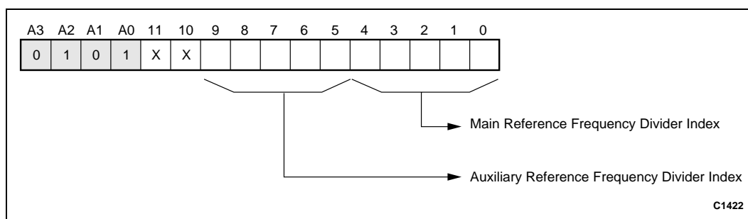
Figure 11. Reference Frequency Dividers Register (Write Only)
