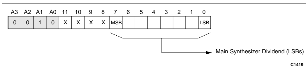
Figure 8. Main Dividend LSB Register (Write Only)
