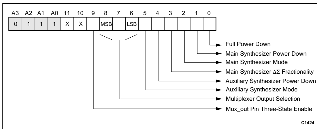
Figure 13. Power Down and Multiplexer Output Register (Write Only)
