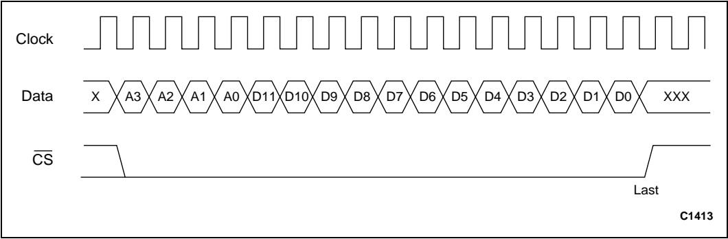
Figure 3. Serial Transfer Timing Diagram
