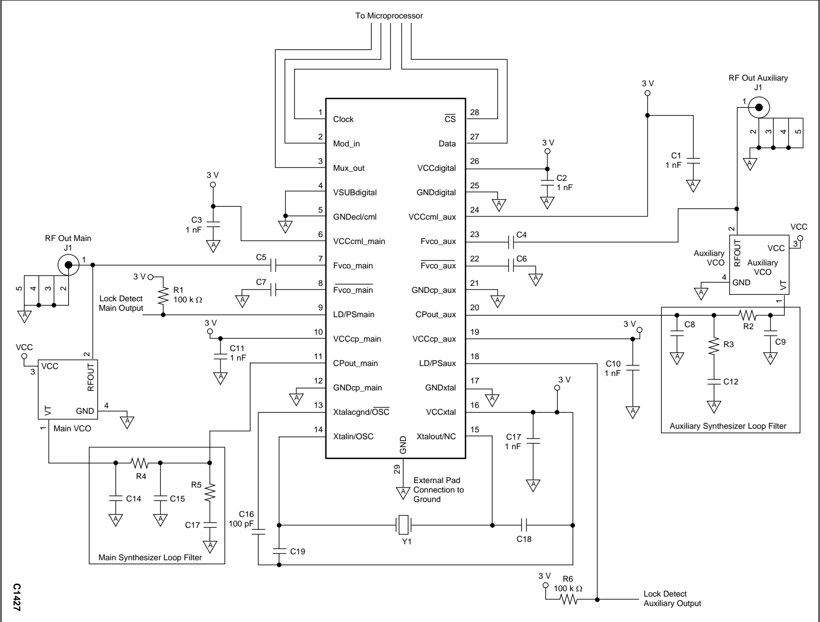
Figure 16. CX72302 Application Schematic
