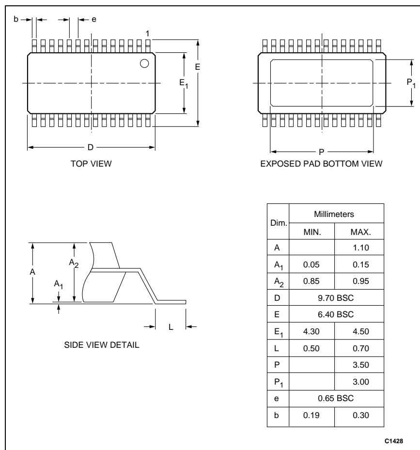
Figure 17. CX72302 28-Pin EP-TSSOP Package Dimension Drawing
