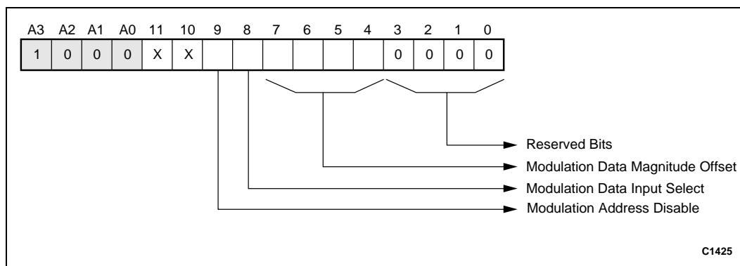
Figure 14. Modulation Control Register (Write Only)
