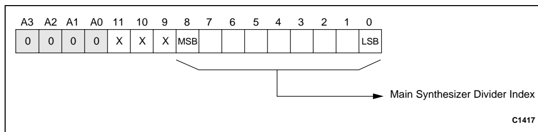
Figure 6. Main Divider Register (Write Only)
