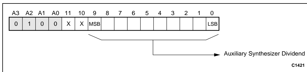
Figure 10. Auxiliary Dividend Register (Write Only)
