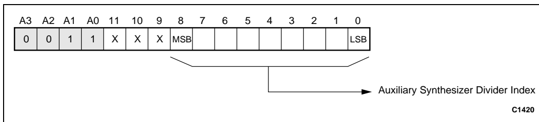
Figure 9. Auxiliary Divider Register (Write Only)
