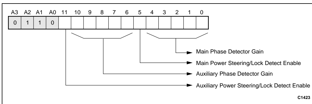
Figure 12. Control Register (Write Only)
