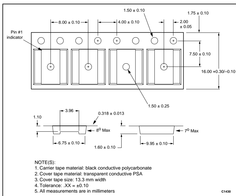
Figure 18. CX72302 Tape and Reel Dimensions
