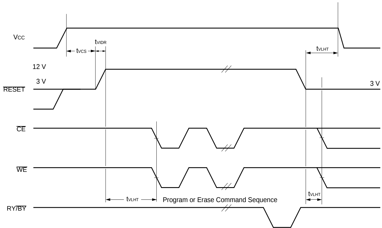
Figure 15 Temporary Sector Unprotection Timing Diagram
