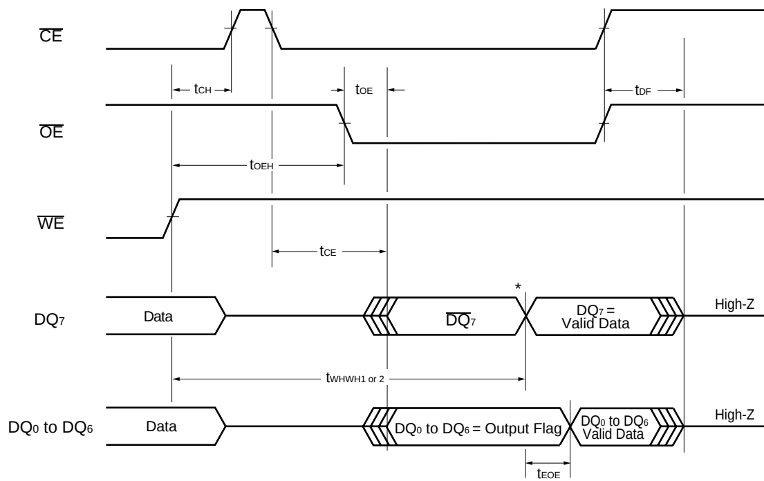
Figure 6 AC Waveforms for \overline{Data} Polling during Embedded Algorithm Operations
