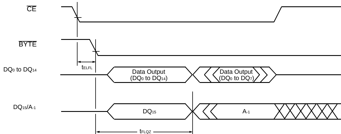
Figure 11 Timing Diagram for Byte Mode Configuration
