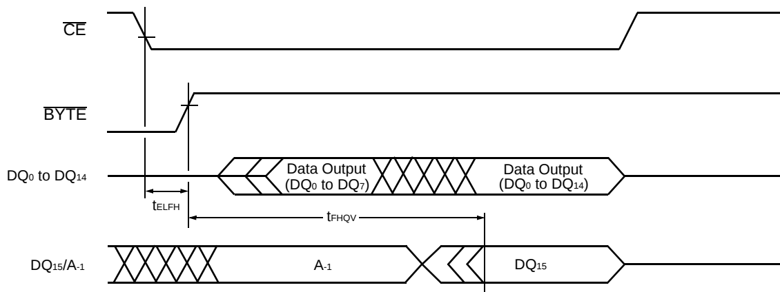
Figure 10 Timing Diagram for Word Mode Configuration
