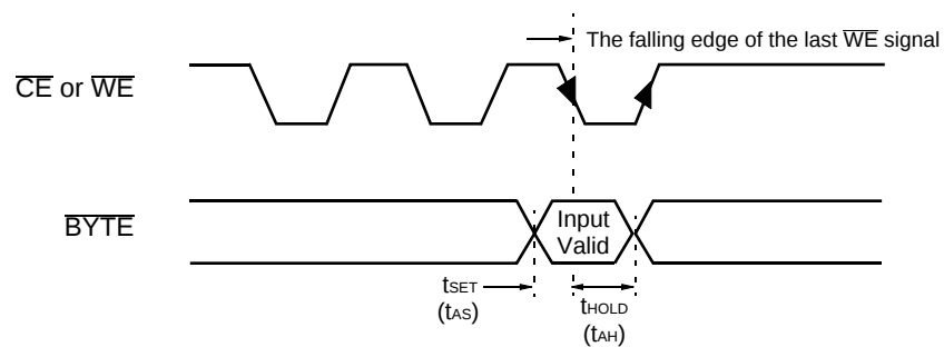
Figure 12 BYTE Timing Diagram for Write Operations
