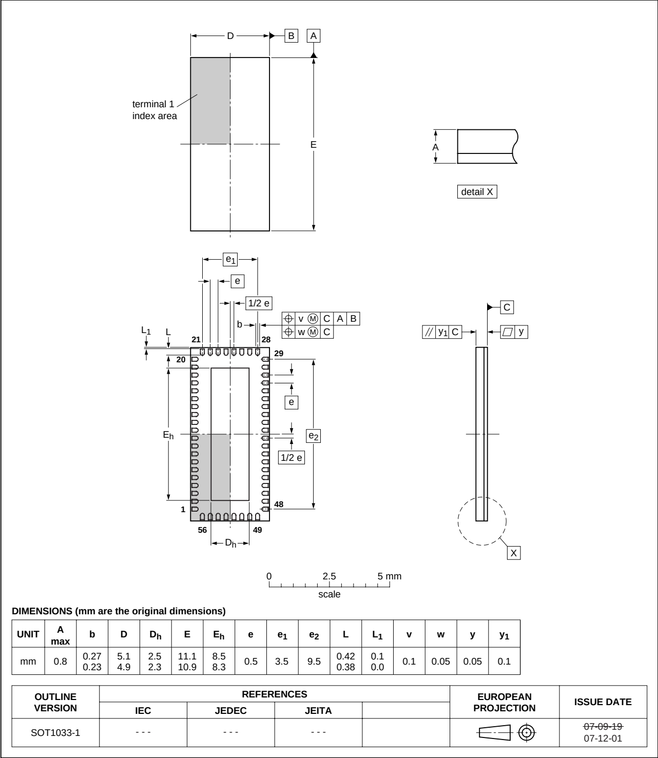
Fig 8. Package outline HWQFN56R (SOT1033-1)
