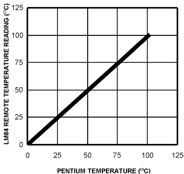
Pentium Temperature vs LM84 Temperature Reading
