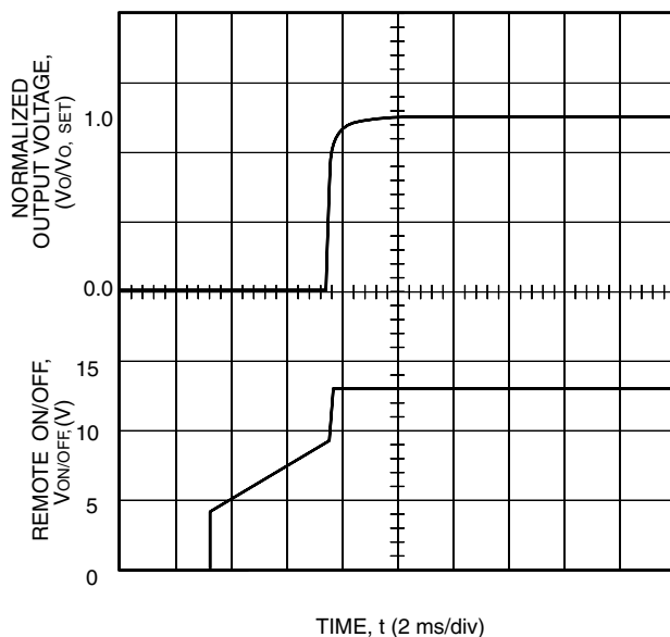
Figure 15. Typical Output Voltage Start-Up when Signal Is Applied to Remote On/Off; I_o = I_{o, max} , V_i = \text{Nominal Line} at T_c = 25^\circ\text{C}
