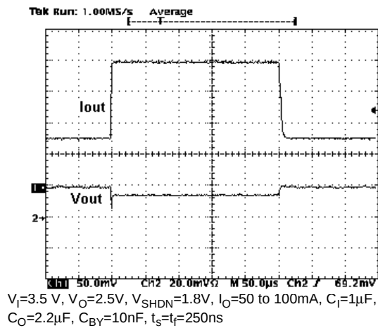
Figure 26 : Load Transient
