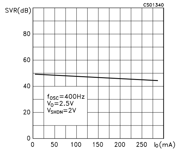
Figure 11 : Supply Voltage Rejection vs Output Current
