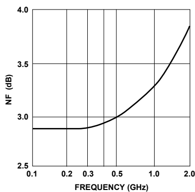
Figure 4. Noise Figure vs. Frequency, I_d = 29 \text{ mA} .
