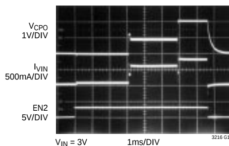
Charge Pump Mode Switching and Input Current
