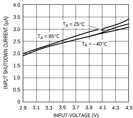
Input Shutdown Current vs Input Voltage
