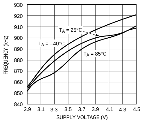
Oscillator Frequency vs Supply Voltage
