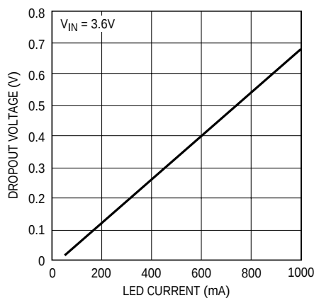
I_{LED} Dropout Voltage vs LED Current
