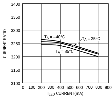
I_{SET}/I_{LED} Current Ratio vs I_{LED} Current
