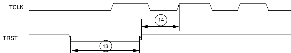
Figure 13. \overline{\text{TRST}} Timing
