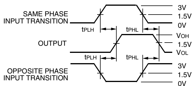
Propagation Delay
