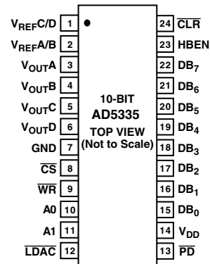
AD5335 PIN CONFIGURATION
